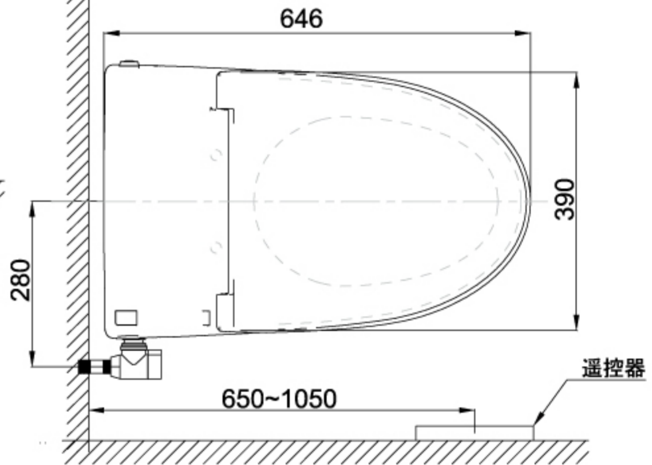
TOP VIEW
