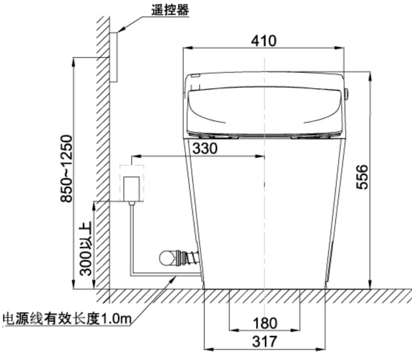
FRONT_VIEW
